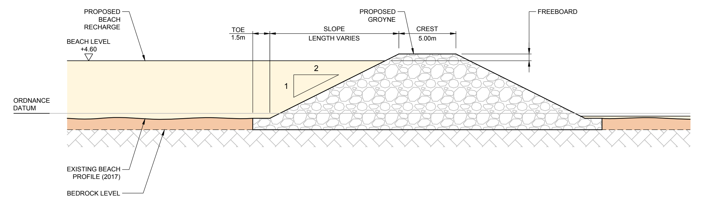
SECTION A-A THROUGH PROPOSED GROUPE (SCHEMATIC) SCALE 1:200
