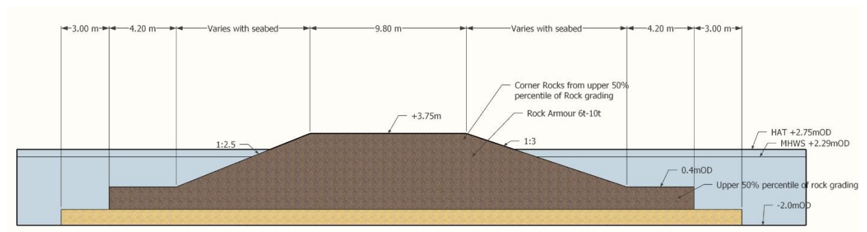
Figure 4-10: Sketch of eastern breakwater in front of East Beach
