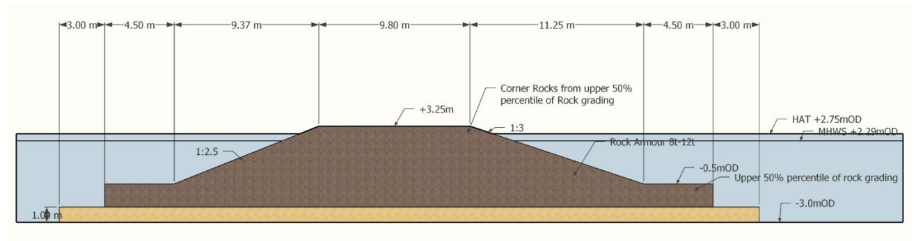
Figure 4-8: Sketch of town beach breakwaters according to Layout 3
